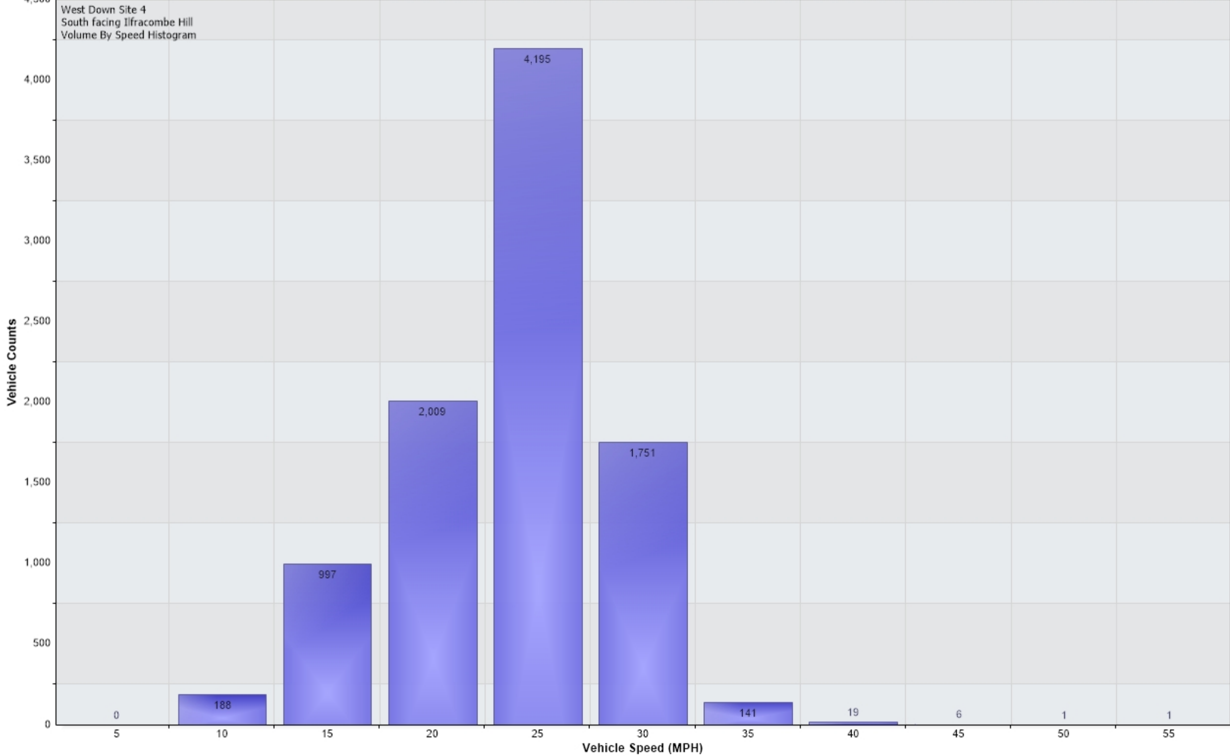
Vehicle Counts Vs. Speed [West Down Site 4: Incoming]
